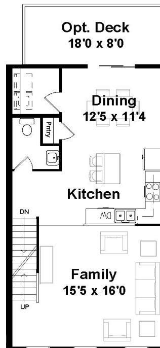
Second Floor 8ft Ceilings Options Shown: Kitchen Island
