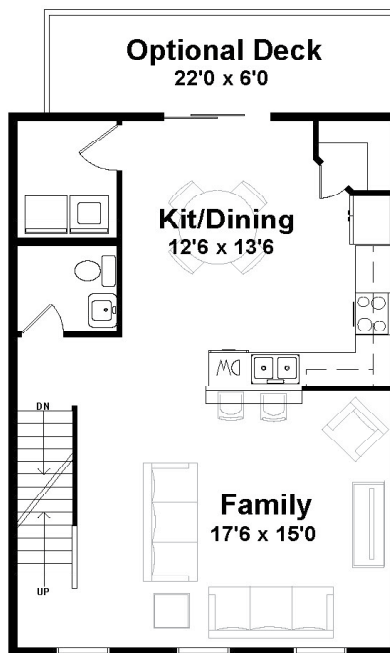
Second Floor Options Shown: Kitchen Pantry, and Kitchen Half Wall Countertop
